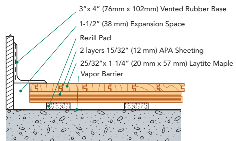
WALL BASE DETAIL (RezillPanel)
