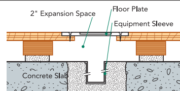
EQUIPMENT DETAIL (optional accessory)
