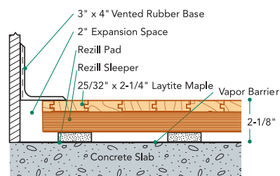
WALL BASE DETAIL (RezillSleeper)
