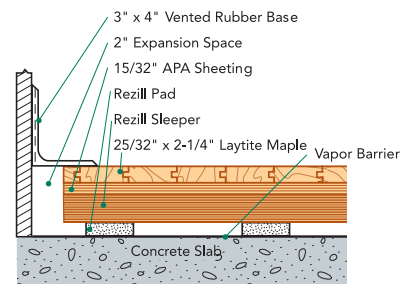
WALL BASE DETAIL (RezillSleeper Subfloor)
